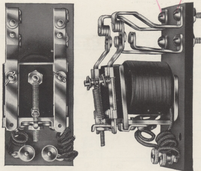
Illustration of FB6 Relay.
